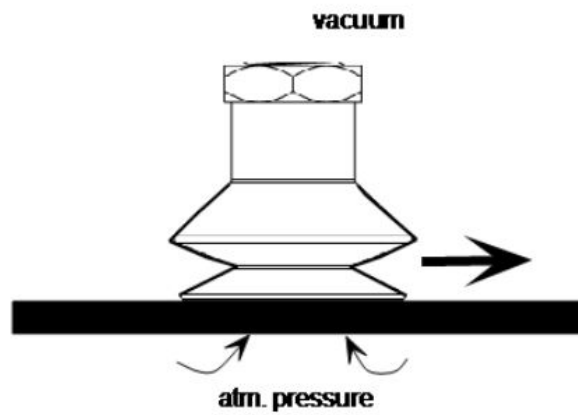
Fig. 6-16: Non-porous material
